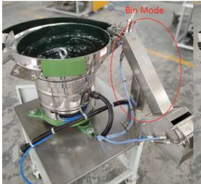
Bin mode vibration bowl
