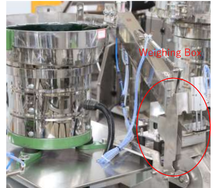
Vibration bowl with weighing box
